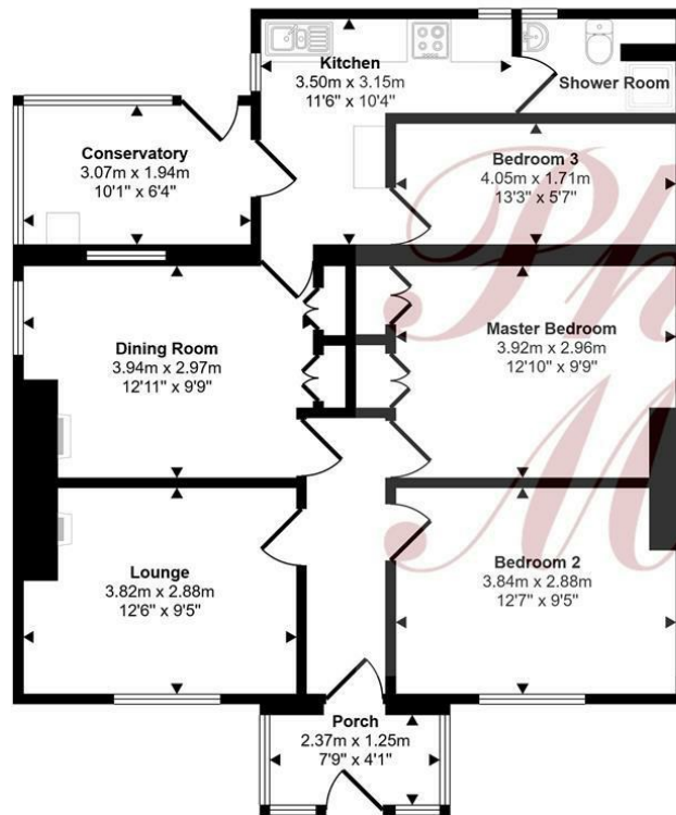
Ground Floor Approx 86 sq m / 929 sq ft
